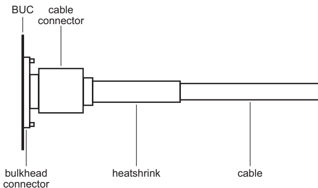
Figure 2: Sealed connector
