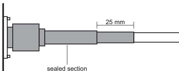
Figure 2: Sealed connector
